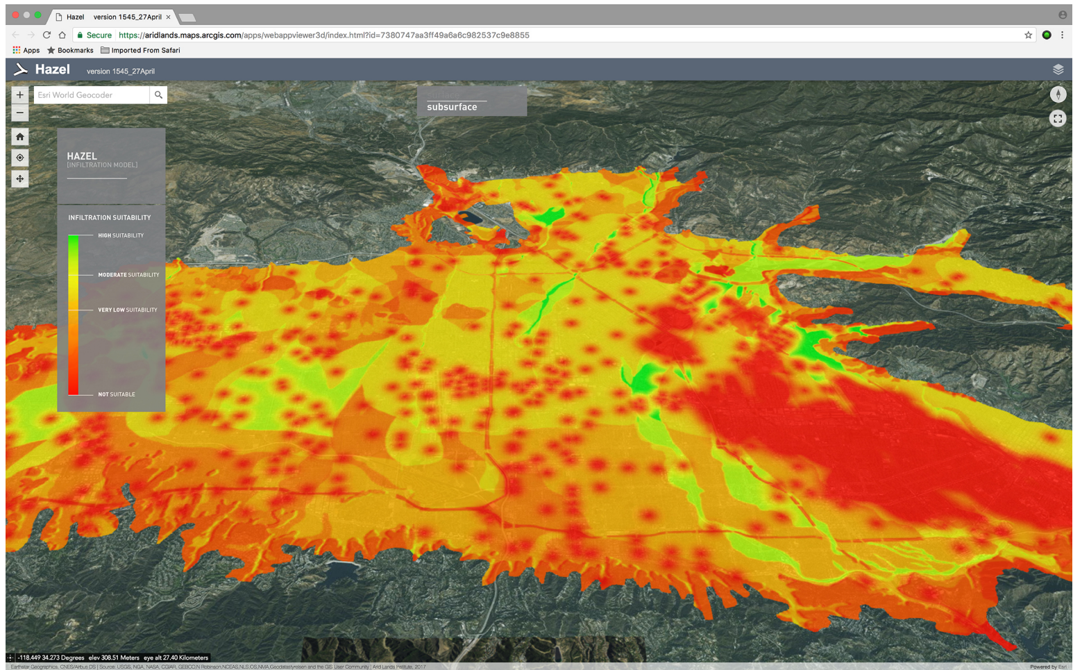
Figure 4: Hazel subsurface infiltration suitability across a 200 mi 2 study area.
