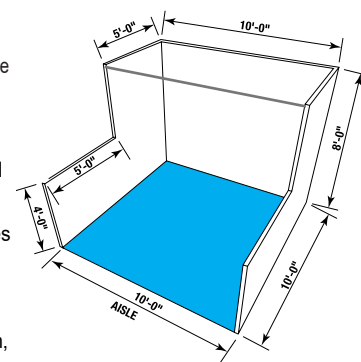
In-Line (Linear) Booth with Canopies or Ceilings
